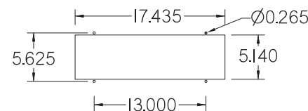
CONTROL PANEL CUTOUT
